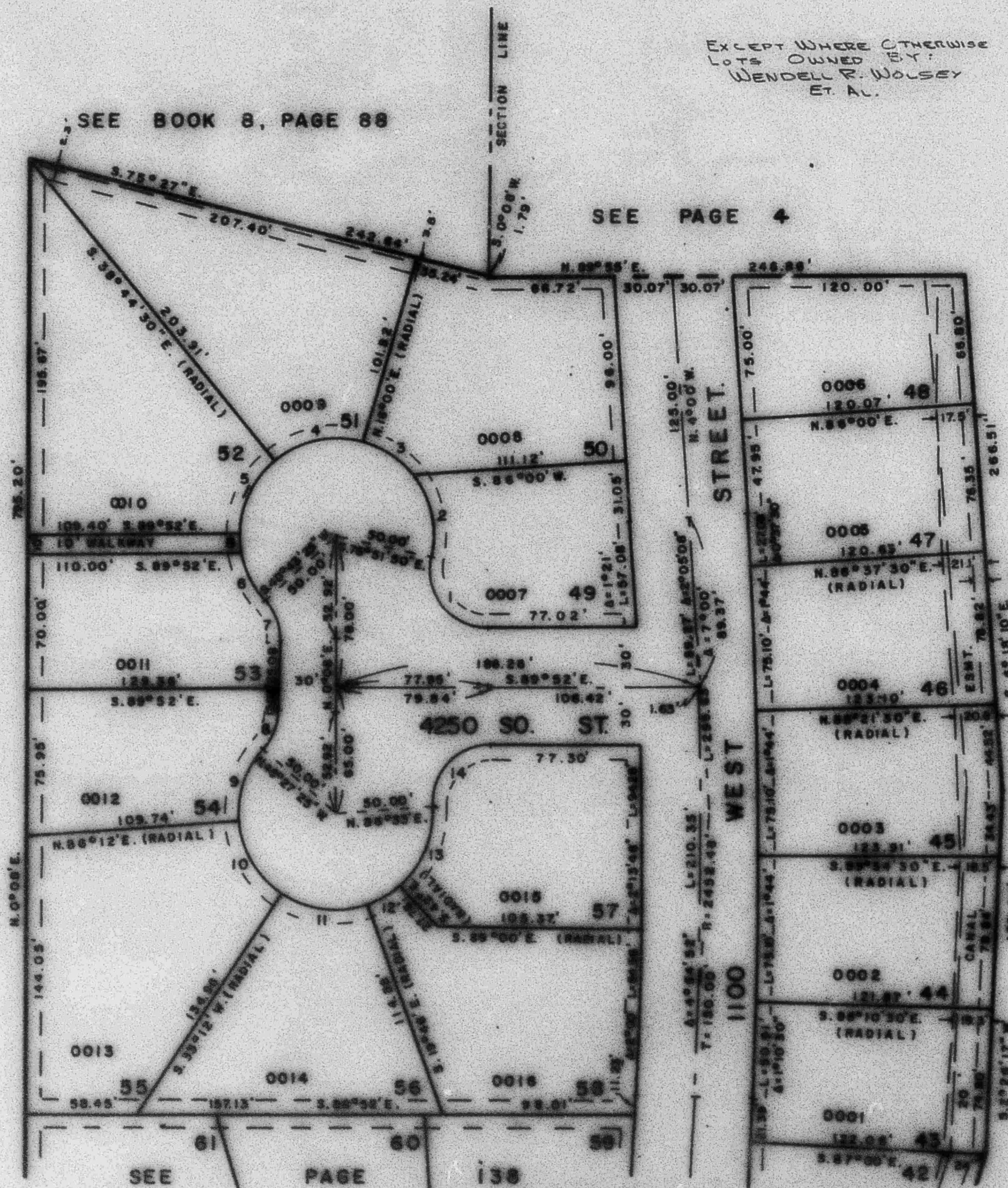
CURVE DATA
